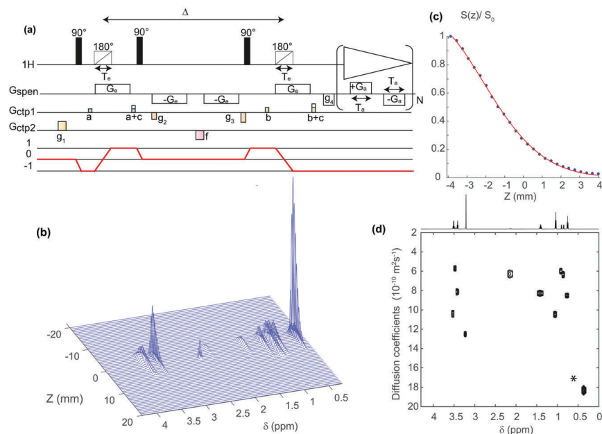
Fig. 2 SPEN 2D DOSY. (a) Pulse sequence for SPEN 2D DOSY. The selected coherence transfer pathway is shown in red. Gradients a and b are crushers surrounding the refocusing chirp pulses; gradient c selects the anti-echo pathway for the stimulated echo; gradient f is a spoiler during longitudinal storage; g 1 , g 2 and g 3 are compensating gradients. (b) 2D spectroscopic imaging data set obtained with the SPEN 2D DOSY experiment on a mixture of 3 alcohols (methanol, ethanol, propanol) and an amino-acid (L-valine), at a concentration of ~100 mM in D 2 O. (c) Diffusion decay curve obtained from the data set shown in (b), for the methanol CH 3 resonances at 3.2 ppm. The best fit-curve for the modified Stejskal–Tanner equation is shown in red with D = 12.5 \times 10^{-10} \text{ m}^2 \text{ s}^{-1} (d) 2D DOSY display obtained from the data set shown in (b), the average diffusion coefficients are 18.4 \times 10^{-10} \text{ m}^2 \text{ s}^{-1} for water, 12.5 \times 10^{-10} \text{ m}^2 \text{ s}^{-1} for methanol, 10.3 \times 10^{-10} \text{ m}^2 \text{ s}^{-1} for ethanol, 8.5 \times 10^{-10} \text{ m}^2 \text{ s}^{-1} for propanol and 6.1 \times 10^{-10} \text{ m}^2 \text{ s}^{-1} for L-valine. The water peak is folded and indicated by an asterisk. The 1 H pulse-acquire spectrum is shown above the DOSY display. The experiment was carried out with a 600 MHz spectrometer equipped with a triple-axis gradient high-resolution probe.
