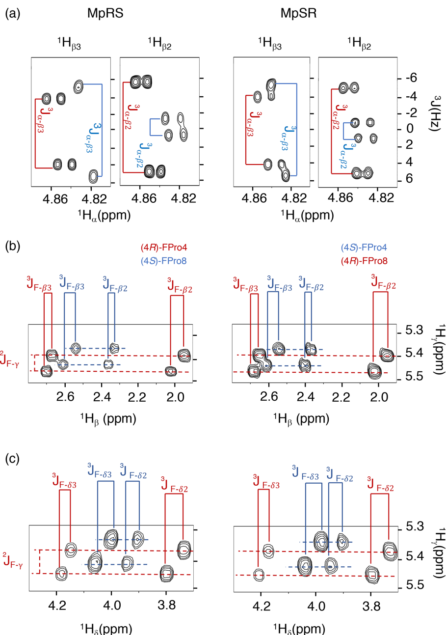
Figure 3. Puckering analysis of fluoroprolines. (a) Homonuclear coupling constants ^3J_{H\alpha-H\beta2} and ^3J_{H\alpha-H\beta3} of the (4R) (in red) and (4S) (in blue) fluoroprolines in MpSR and MpRS peptides measured from SERF experiments at 298 K. (b) The ^3J_{F-H\beta} heteronuclear coupling constants extracted from 2D ^1H - ^1H TOCSY spectra using the E.COSY cross-peak pattern. (c) The ^3J_{F-H\delta} heteronuclear coupling constants extracted from 2D ^1H - ^1H TOCSY spectra using the E.COSY cross-peak pattern.
