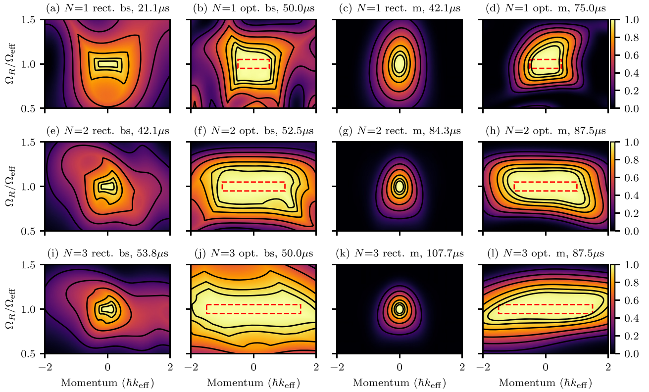
Figure 5. Simulated state-transfer fidelities of rectangular ((a), (c), (e), (g), (i) and (k)) and optimized ((b), (d), (f), (h), (j) and (l)) symmetric Raman pulses for momentum orders of N = 1, 2 , and 3 shown as a function of initial atomic momentum on the x -axis and the amplitude error on the y -axis. Beamsplitter (bs) pulses are shown in the first two columns; mirror (m) pulses are shown in the final two. For the optimized pulses the region of optimization is indicated by the red dashed box. The contours are at 0.2, 0.4, 0.6, 0.8, 0.9 , and 0.95 . Axis labels include the total duration of each composite pulse sequence showing that, as N is increased, optimized sequences can be significantly shorter than their rectangular counterparts.
