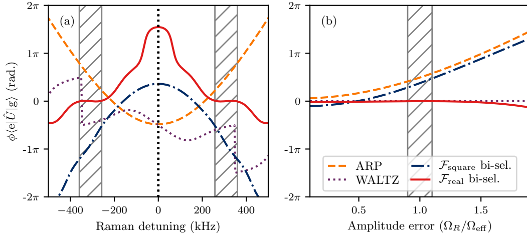
FIGURE 9.5: Phase of overlap \langle e|\hat{U}|g\rangle for different pulses as a function of the Raman detuning (a) and amplitude error (b). The solid red and dot-dashed blue curves correspond to the 10 th \mathcal{F}_{\text{real}} and \mathcal{F}_{\text{square}} bi-selective pulses, respectively. The orange dashed curve represents the tanh/tan pulse of the same duration ( 4t_\pi ) and the purple dotted curve shows the results for WALTZ. The hatched regions represent the design ranges in detuning and amplitude errors over which the phase is minimised when using \mathcal{F}_{\text{real}} . In (a) \Omega_R = \Omega_{\text{eff}} and in (b) the detuning corresponds to the centre of the Doppler-shifted resonance of the upper interferometer arm during the 10 th augmentation pulse. The curves have been unwrapped and a uniform phase shift has been applied to enhance visual clarity.
