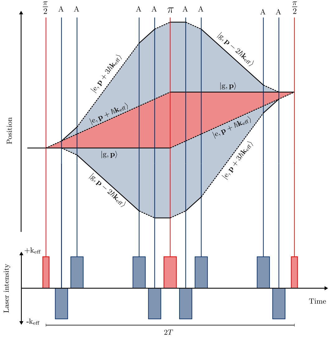
FIGURE 3.6: Positions of atomic trajectories as a function of time for a three-pulse Mach-Zehnder interferometer and a LMT interferometer, where the beamsplitter and mirror operations are each extended by a sequence of 2 augmentation pulses ( N = 2 ), which we label A in the diagram. By increasing the enclosed area of the interferometer the scale-factor and hence intrinsic sensitivity is increased. Solid and dotted lines represent atoms in the internal states |g\rangle and |e\rangle respectively.
