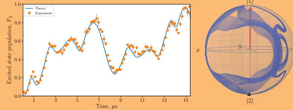
Figure 3: Temporal evolution of atoms (left) and simulated Bloch sphere trajectories (right) for two GRAPE pulses showing optimised state transfer in a \sim 30\mu\text{K} cloud. Our model has good agreement with the data, demonstrating optimal control theory works for our system.
