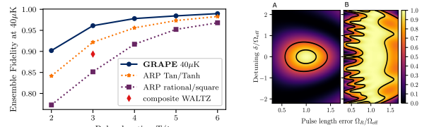
Figure 3: (left) Simulated average pulse efficiency in a 40\mu\text{K} atom cloud for different augmentation pulses as a function of pulse duration as a fraction of that for a rectangular \pi pulse. GRAPE offers more efficient and shorter pulses than composite [4] and Adiabatic Rapid Passage (ARP) alternatives [5-7]. (right) Simulated efficiency of GRAPE inversion pulse (A) and rectangular \pi pulse (B) computed for off-resonance and pulse-length errors.
