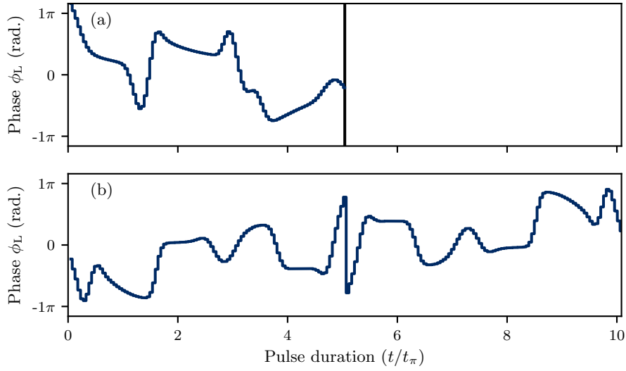
FIGURE 8.9: Optimisation results for a PP 90^\circ beamsplitter pulse (a), and an anti-symmetric UR 180^\circ mirror pulse (b). The pulse profiles are plotted against time as a fraction of the duration of a rectangular \pi pulse, t_\pi . Each optimisation was continued until fidelities greater than 0.99 were reached. Each pulse was optimised for an ensemble of atoms with a temperature of 120\ \mu\text{K} and a range of coupling strengths of \pm 10\% \Omega_{\text{eff}} . \Omega_{\text{eff}} , or the effective Rabi frequency, was 420\ \text{kHz} .
