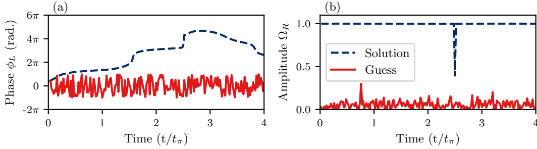
FIGURE 7.15: Initial and final waveform for a \mathcal{F}_{\text{square}} pulse optimised for a temperature of 40 \mu\text{K} and a range of pulse-length errors of \pm 10\% \Omega_{\text{eff}} . Both the laser phase (a) and amplitude (b) were allowed to vary and the SNS penalty was imposed to keep the Rabi frequency from exceeding \Omega_{\text{eff}} .
